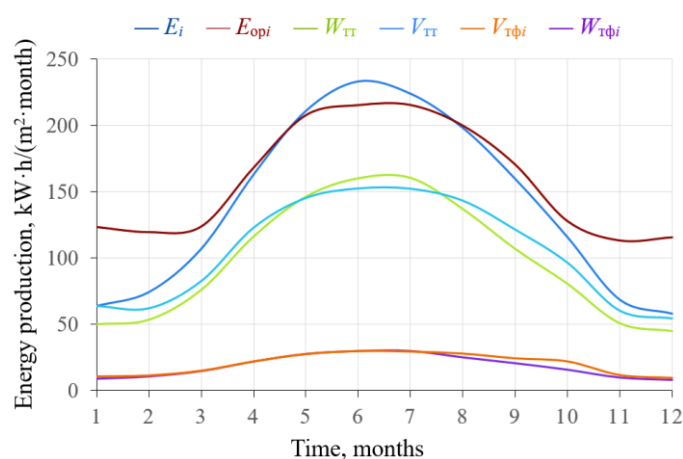
Fig. 2. Distribution of solar energy resource potentials: gross E_{opi} and technical E_i , converted into thermal W_{tr} and electrical energy W_{\phi i} specific production into thermal V_{tr} and electrical V_{\phi} energy on the territory of the island by month during the year
