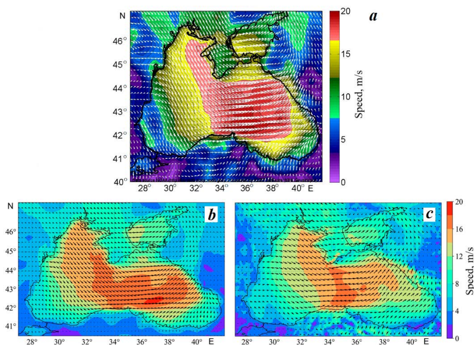
F i g . 2 . Examples of presentation of the wind fields on 3 December 2016: a – from satellite data ( http://dvs.net.ru/mp/data/vel/jpg/wind/wind_nomads_2016120306.jpg ); b – from ERA5 data; c – from SKIRON data
