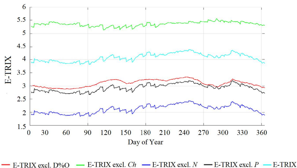
Fig. 3. Contribution of individual hydrochemical characteristics to E-TRIX quantity
