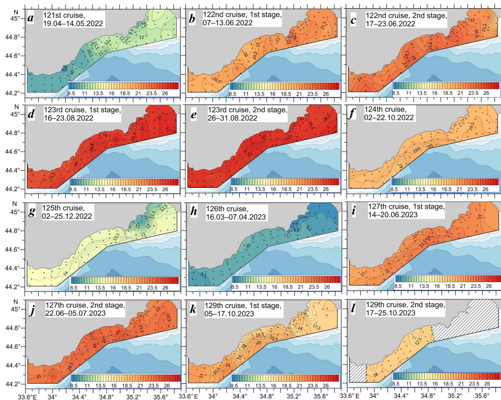
Fig. 2. SST distribution according to the measurements carried out in the 121 st (a), 122 nd (b, c), 123 rd (d, e), 124 th (f), 125 th (g), 126 th (h), 127 th (i, j) and 129 th (k, l) cruises of R/V Professor Vodyanitsky
